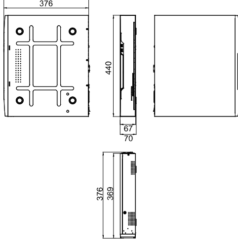
Figure 2-1 Dimensions (Unit:mm)
